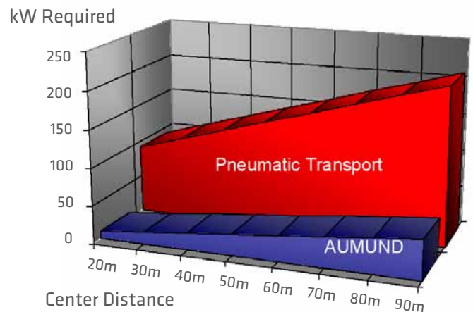
FIGURE 3 Energy consumption for Pneumatic Transport vs Aumund System (based on 200 tph)
