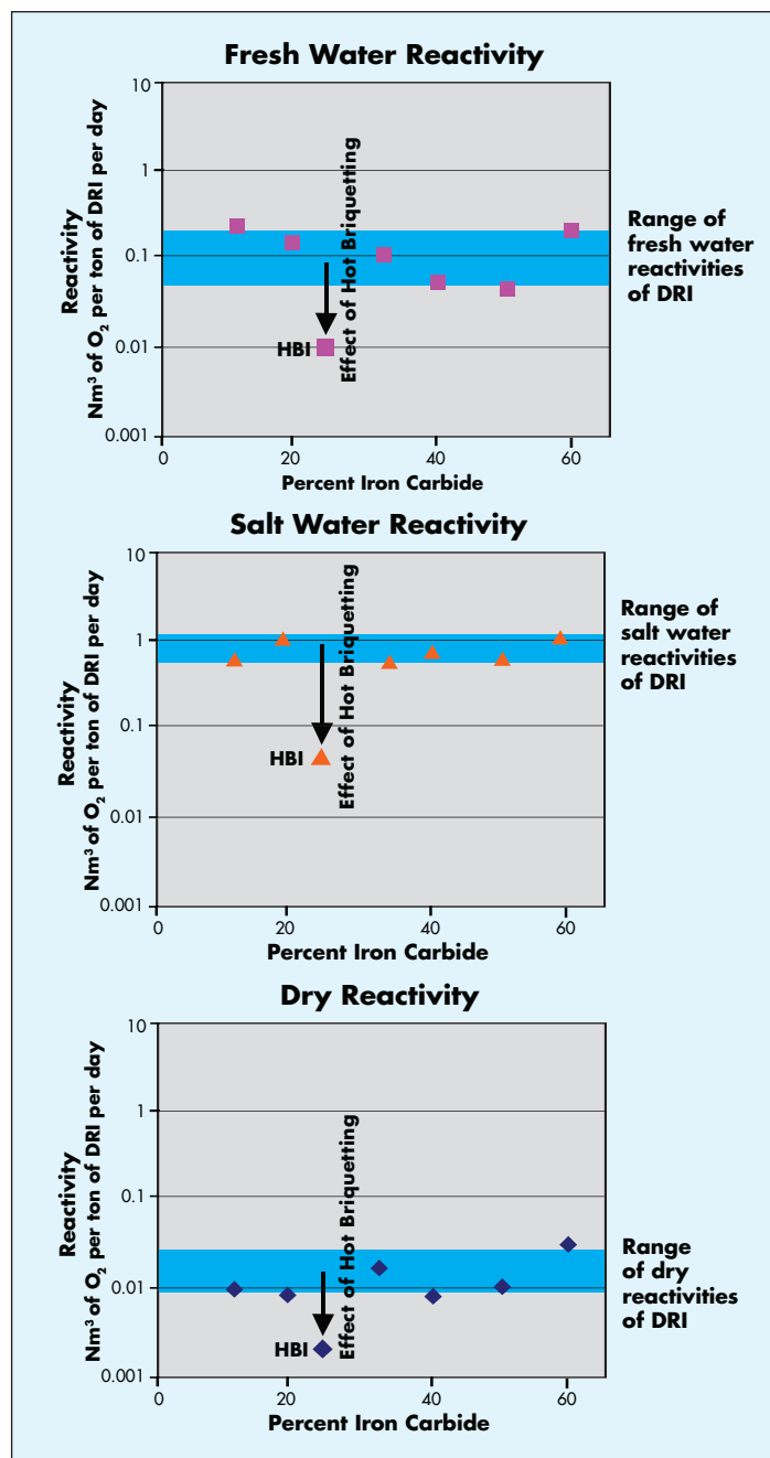
Figure 2- Comparison of HBI Reactivity to the Reactivity of DRI (containing various quantities of Iron Carbide)
