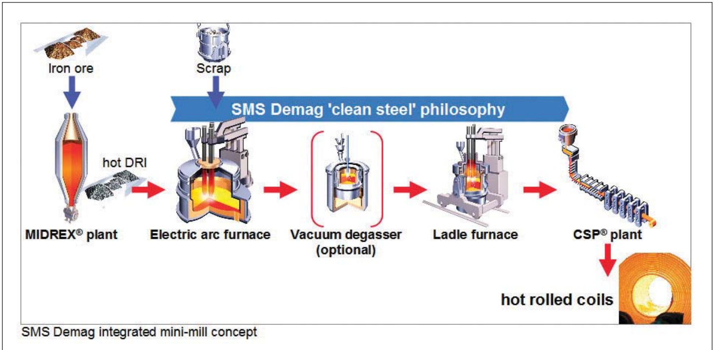
Figure 1 – Integrated Mini-Mill Concept
