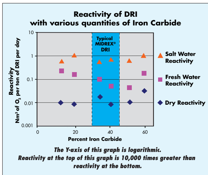
Figure 1 - DRI Reactivity vs. Iron Carbide Content
