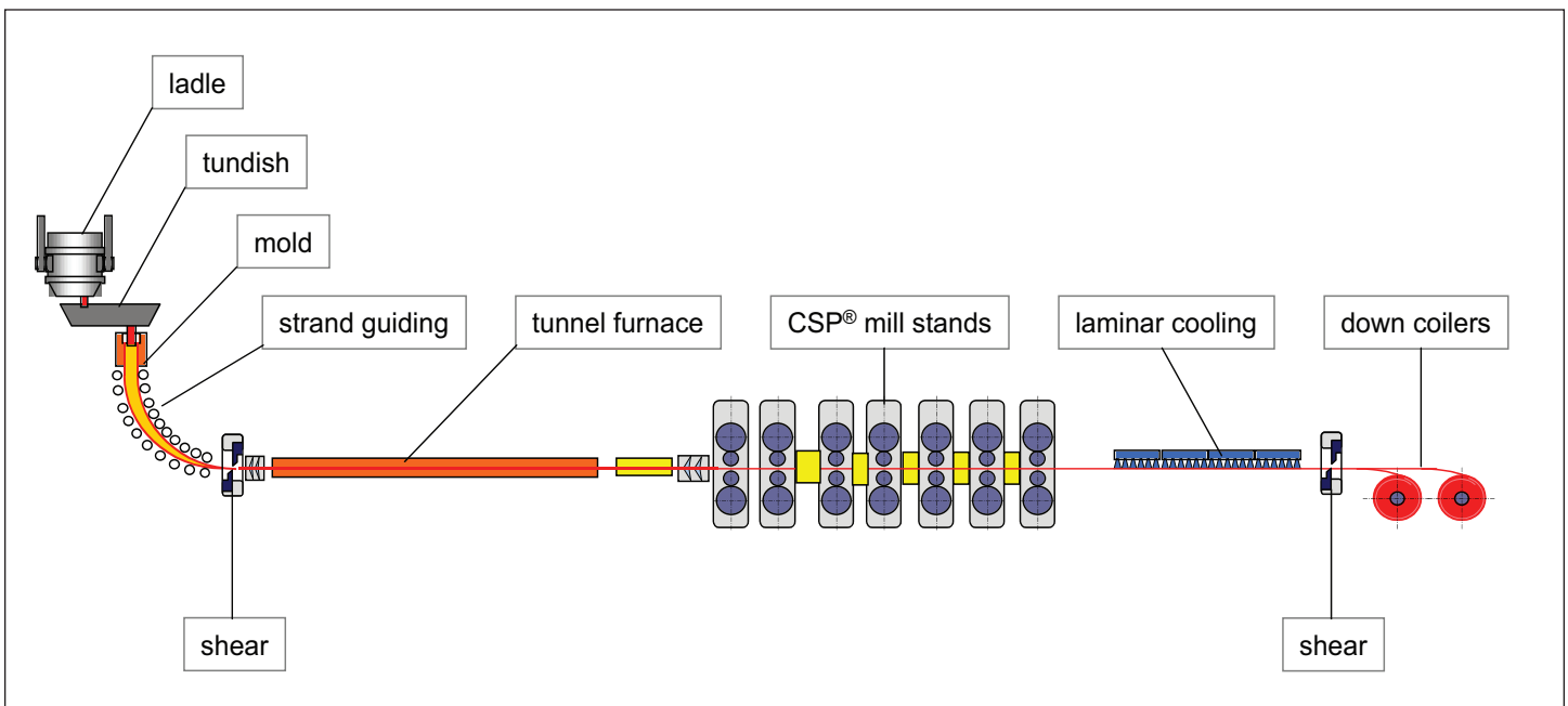
Figure 2 - CSP® Flowsheet
