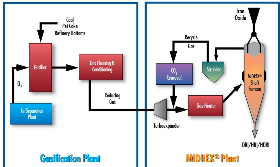
FIGURE 3 MXCOL Flowsheet
